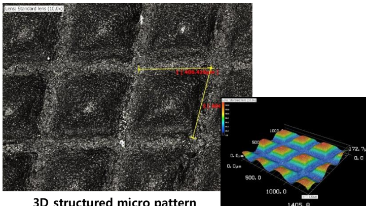
3D structured micro pattern
